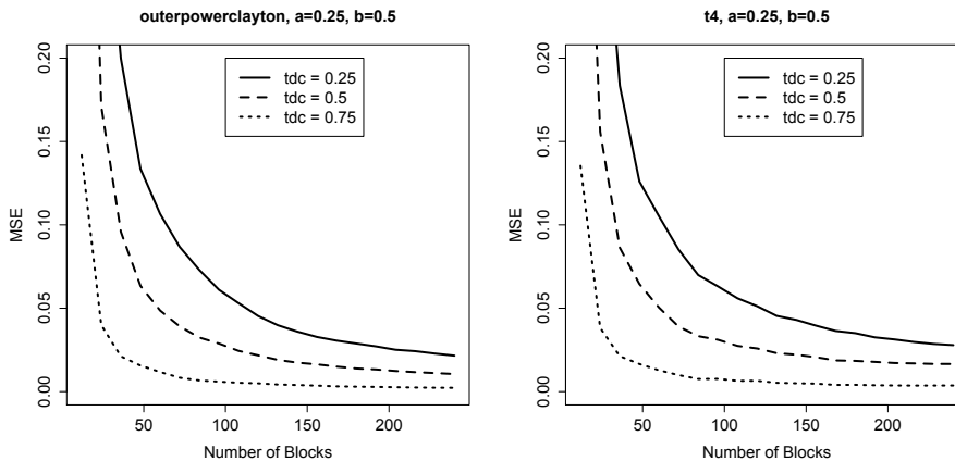
Figure 2: Simulation results for MSE^{(sum)} , with fixed m = 30 . Left: outpower transform of a Clayton copula, right: t_4 -copula, both with parameter chosen in such a way that the coefficient of upper tail dependence is given by 0.25 (solid lines), 0.5 (dashed lines) or 0.75 (dotted lines).
