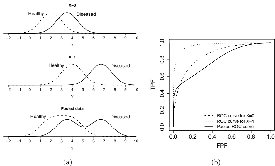
Figure 2: (a) Probability distributions of Y in diseased (solid line) and healthy (dashed line) populations conditional on \mathbf{X} and pooled probability distributions. (b) Conditional ROC curve in each of the populations determined by covariate \mathbf{X} , together with the pooled ROC curve. The shown results were obtained assuming that the performance and discriminatory capacity of the diagnostic test depend on \mathbf{X} , but \mathbf{X} is independent of true disease status: P(\text{status } D \mid \mathbf{X} = 1) = P(\text{status } D \mid \mathbf{X} = 0) = 0.5 . Moreover, P(\text{status } D) = 0.5 and P(\mathbf{X} = 1) = 0.5 were considered.
