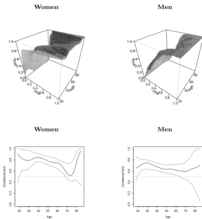
Figure 4: Estimated conditional ROC curves and AUCs for the endocrinology data for women and men. The dashed lines represent the 95 per cent pointwise bootstrap confidence interval.
