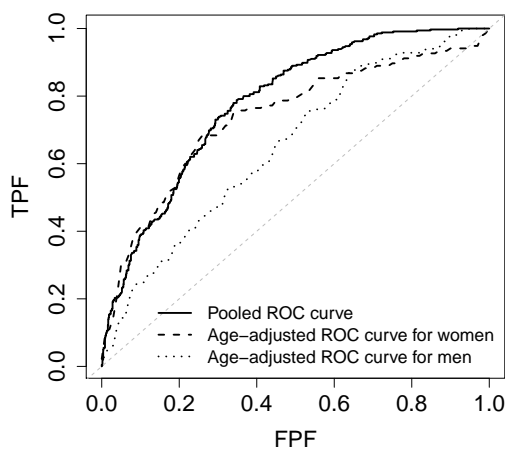
Figure 3: Estimated pooled ROC curve for the endocrinology data (solid line). The dashed and dotted lines represent the estimated age-adjusted ROC curve for women and men, respectively.
